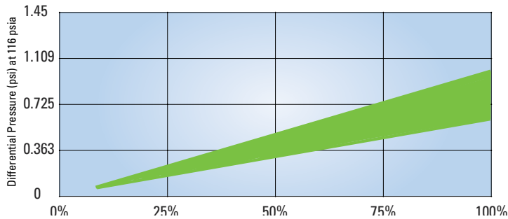
DF-C Cyclone Separator Differential pressure related to nominal flow rate
