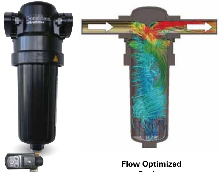
DF-C Standard with UFZ time controlled condensate drain
